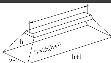
25.picture: Explanation of heat-radiated area
