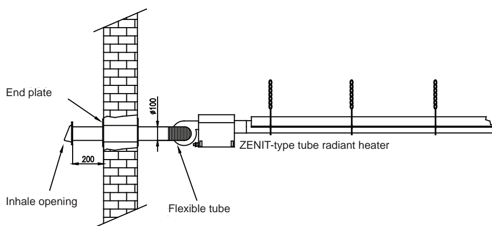
31.picture: Outside combustion-air supply
